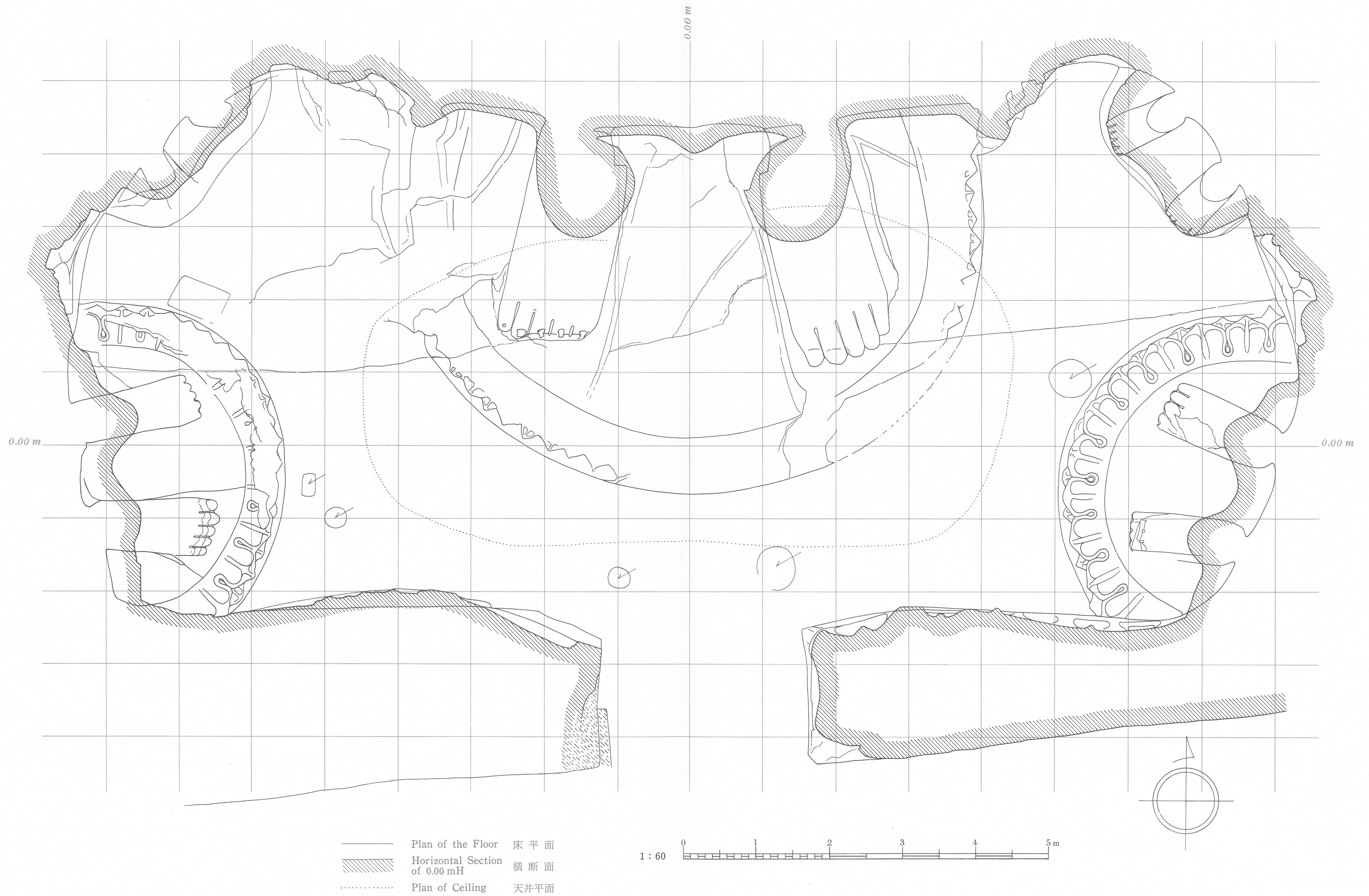
HORIZONTAL SECTION CAVE XVIII
